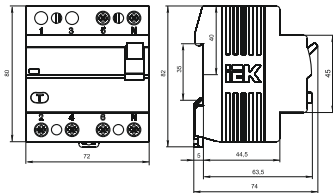
Figure 2 – Overall and installation dimensions of four-polar VDs
